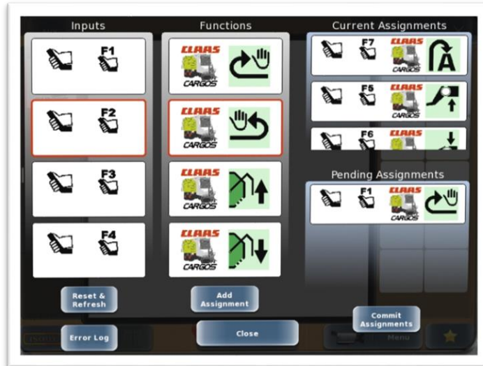
Externes ISOBUS - Terminal
