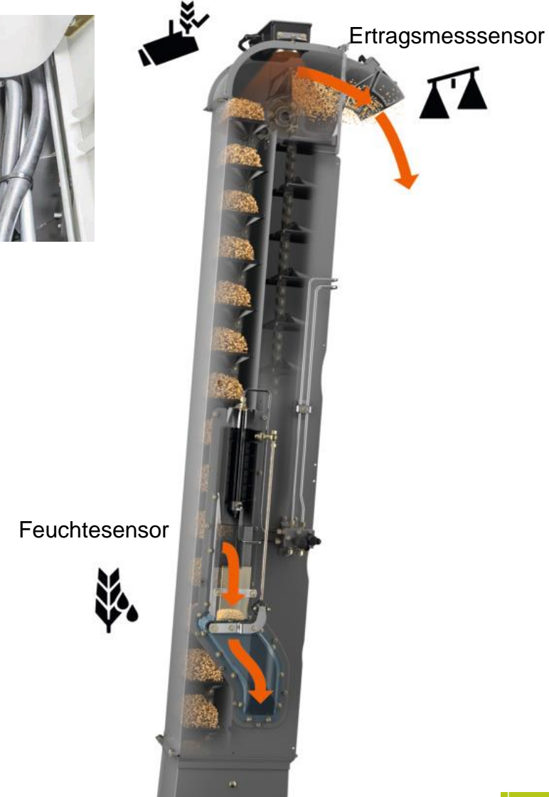
GRAIN QUALITY CAMERA
