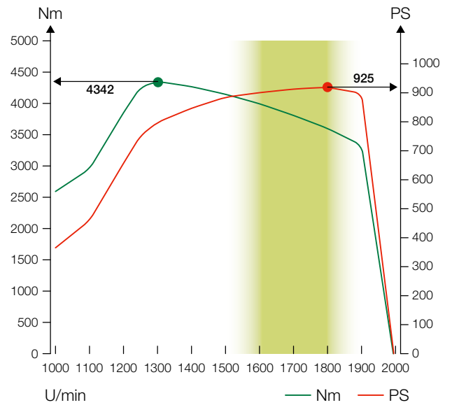
High engine output - JAGUAR 990.
