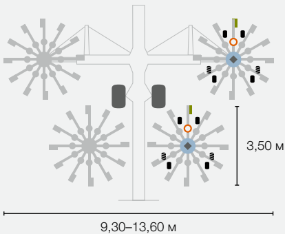
LINER 4800 BUSINESS / LINER 4800 TREND
